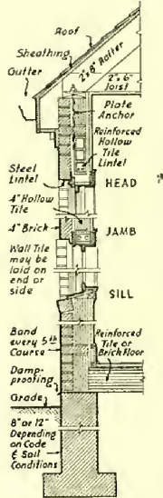
Wall Section
